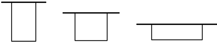
Branta coffee tables powder coated stainless steel/ceramic or HPL Ø55 h49, Ø70 h35, Ø100 h20 cm
